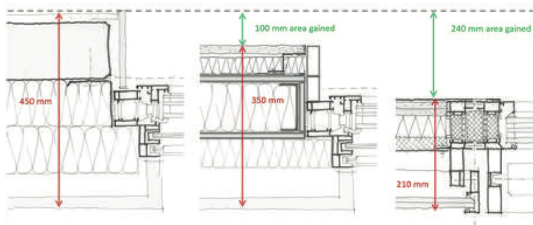
FIG. 6 Comparison of the net floor area gain (green arrow) by the application of ultra-slim façade systems
