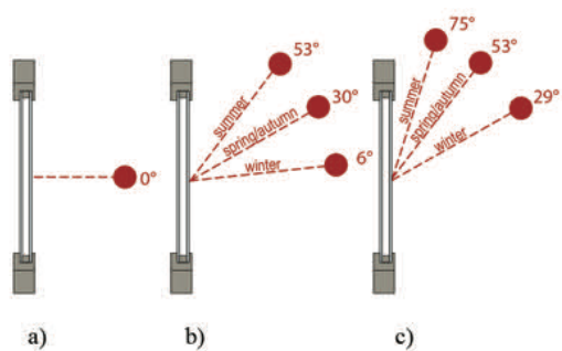
FIG. 6 Angle of incidence for solar radiation for a) at 0° (normal incidence) for product (standardised) measurements and actual incidence angle for b) Helsinki and c) Athens for different seasons of the year
