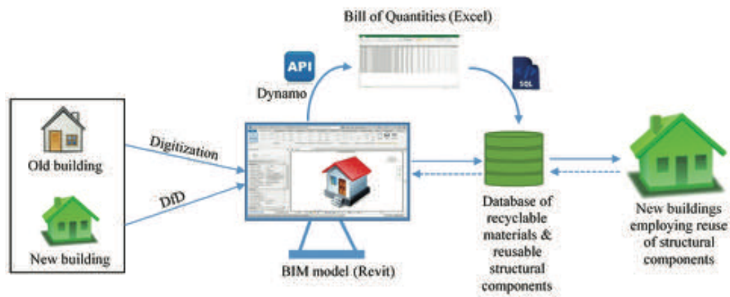
FIG. 4 The representation of BIM-coupled digital M&C bank
