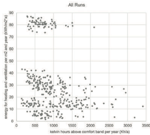
FIG. 5 Point cloud of all simulation runs accordingly to the criteria energy demand and summery overheat hours per year
