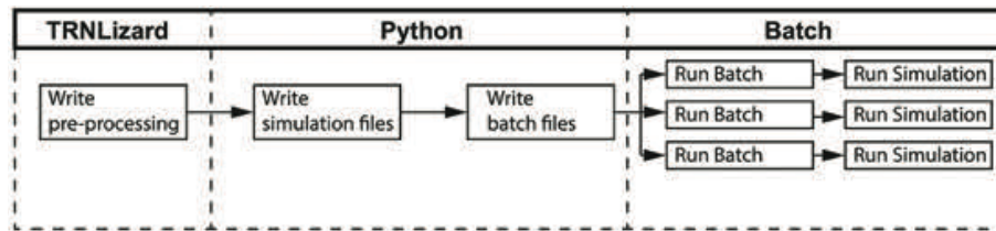
FIG. 2 Parallelisation methodology
