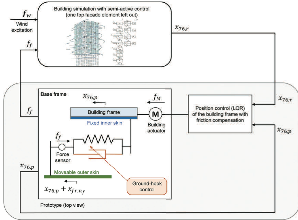
FIG. 8 Hardware in the Loop (HiL) simulation
