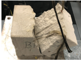
FIG. 11 Pull-out test to determine the adhesion of basalt roving / cementitious foam
