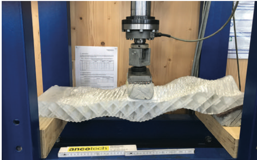
FIG. 5 Design of the experimental unit with test specimen, distributor plate and support forms
