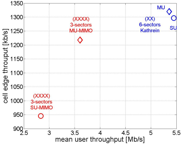
Fig. 6. Hard-Sectorization based on (XXXX) system: mean and edge user throughput for different net work configurations with 24 antenna elements per site. The total transmit power per site is kept constant. A spacing of d = 0.5\lambda (tri-sector) and 0.8\lambda (6-sector) is used.
