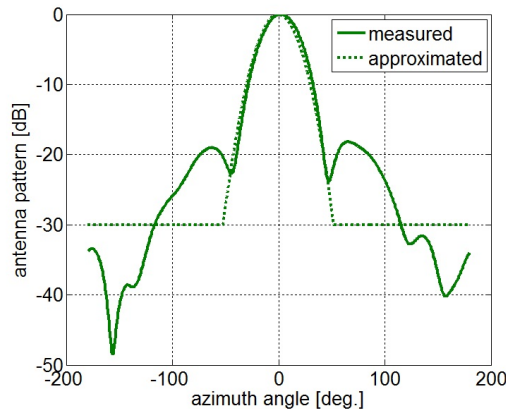
Fig. 1. Measured (solid) antenna pattern in the azimuth direction (Kathrein Type 742351v01) and the approximated (dotted) parabolic pattern using parameters specified in table
