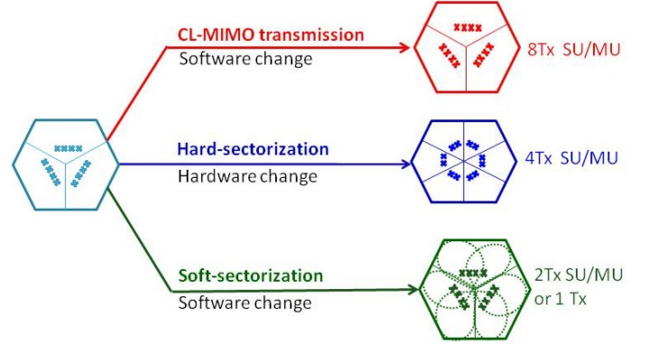
Fig. 5. Different network realizations constraint to 12 pairs of cross polarized antenna elements (24 RF chains) per site (XXXX): CL-MIMO transmission, hard- and soft-sectorization.
