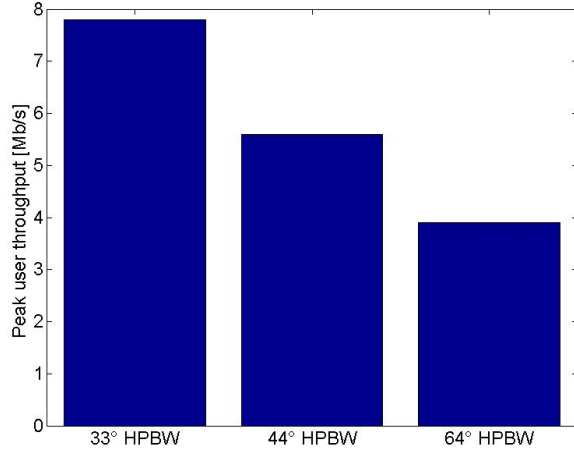
Fig. 3. Peak user throughput for the different network layouts. It doubles as the sector number doubles provided that the beamwidth is properly scaled.
