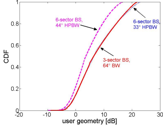
Fig. 2. User geometry distribution for a traditional tri-sector site network with 64° HPBW (solid red) and 6 sector site network using antennas with 33° HPBW (dotted blue) 44° HPBW (dashed magenta). The parameters for the applied antennas are summarized in table I. The red and blue curves are nearly identical. This suggests a doubling in system throughput when switching from 3 to 6 sector site network using the 33° HPBW antennas.
