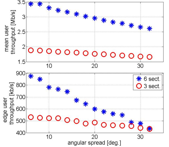
Fig. 4. Mean (top), edge (bottom) user throughput as a function of the azimuth angular spread for a conventional 3-sector and a 6-sector site network applying single transmit antenna (antenna height for BS = 25 m and terminal = 1.5 m). PF scheduler is used. A stronger dependency on the angular spread is observed for higher order sectorized configuration and for edge user throughput. Splitting gain varies between (84-50)% in mean and between (65-0)% in edge user throughput.
