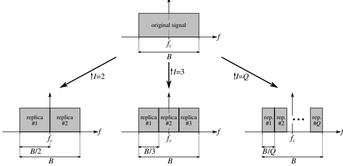
Fig. 3. Ensuring equal spectrum usage for interpolation factors I = 2, 3 and for an arbitrary integer interpolation factor I = Q . I replicas of the interpolated signal are transmitted to ensure that the whole frequency range of the original signal (without interpolation) is used. In this figure the signal bandwidth is denoted by B .
