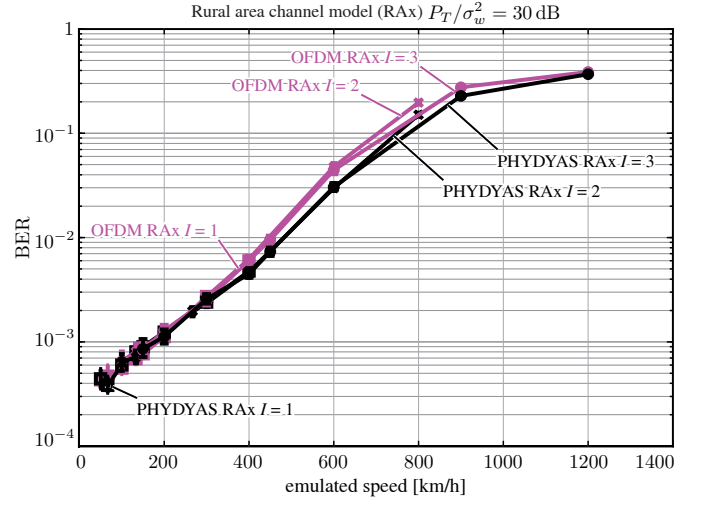
Fig. 5. BER versus emulated speed for OFDM and FBMC with the PHYDYAS prototype filter. RAx channel model and P_T/\sigma_w^2 = 30 dB
