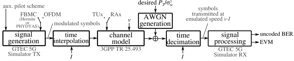
Fig. 2. Block diagram of the setup used for the evaluations.
