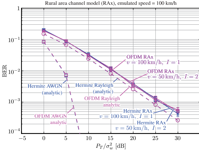
Fig. 4. BER versus P_T/\sigma_w^2 for the RAx channel model.
