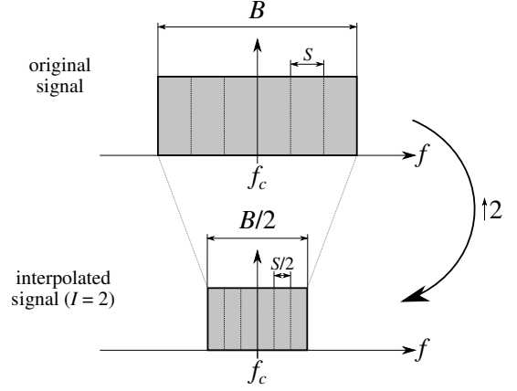
Fig. 1. Example of spectrum compression due to a time interpolation factor I = 2 . It is straightforward to see that the subcarrier spacing S is also reduced by a factor of I since the total bandwidth B is also reduced by the same factor.
