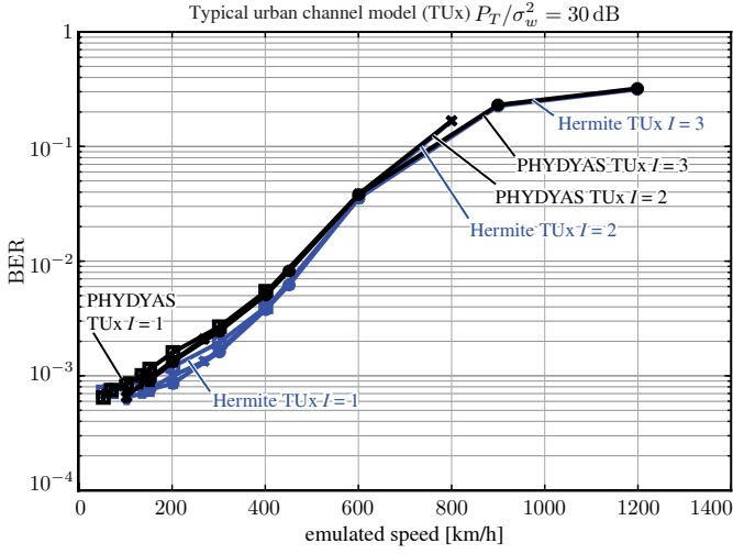
Fig. 7. BER versus emulated speed for the TUx channel model.
