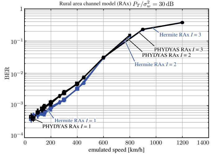
Fig. 6. BER versus emulated speed for FBMC with the PHYDYAS and Hermite prototype filters. RAx channel model and P_T/\sigma_w^2 = 30 dB
