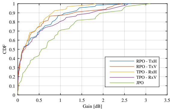
Figure 11. Gain of the polarimetric optimization per beam at different sides.
