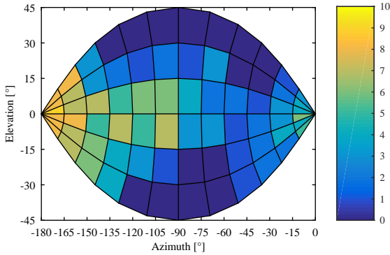
Figure 6. Histogram showing the number of beams distributed in the azimuth and elevation at the Tx.
