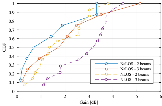
Figure 10. Gain compared to the main beam after adding 2 and 3 beams, considering Tx BF and omni-directional Rx.
