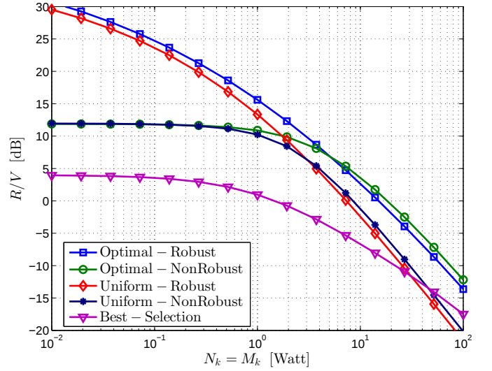
Fig. 5. The behavior of the SNR at the fusion center with respect to the noise powers N_k = M_k for all k is visualized. All curves show an decreasing property in the noise powers.
