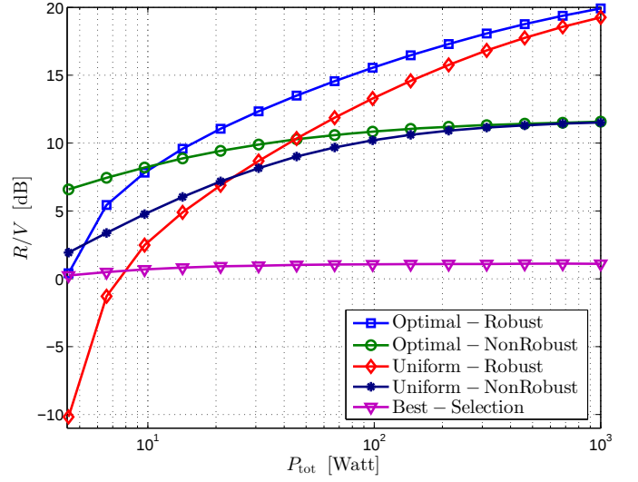
Fig. 3. The behavior of the SNR at the fusion center with respect to the sum power P_{\text{tot}} is visualized. All curves show an increasing property in P_{\text{tot}} .
