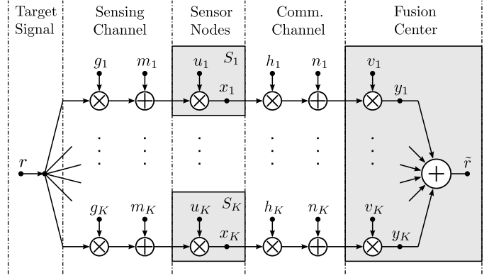
Fig. 1. The system model of the distributed sensor network, which shows the signal flow from a target signal over the sensor nodes to a fusion center.
